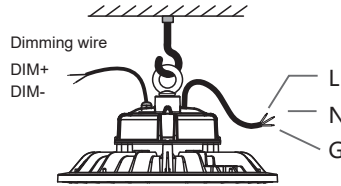
3. Wiring (Dimming Type)
