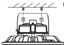
1. Drill holes, fix the expansion screws and then hang the lamp
