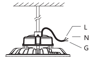
Wiring (Non-dimming Type)
