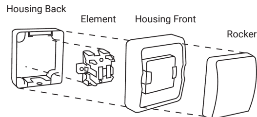
Figure 2 | Change-over switch
