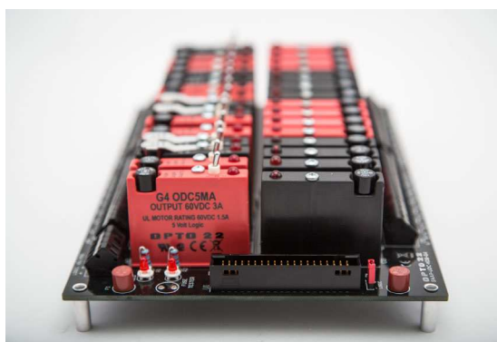
SNAP-UDC-HDB-G4 shown with G4 modules (sold separately)
