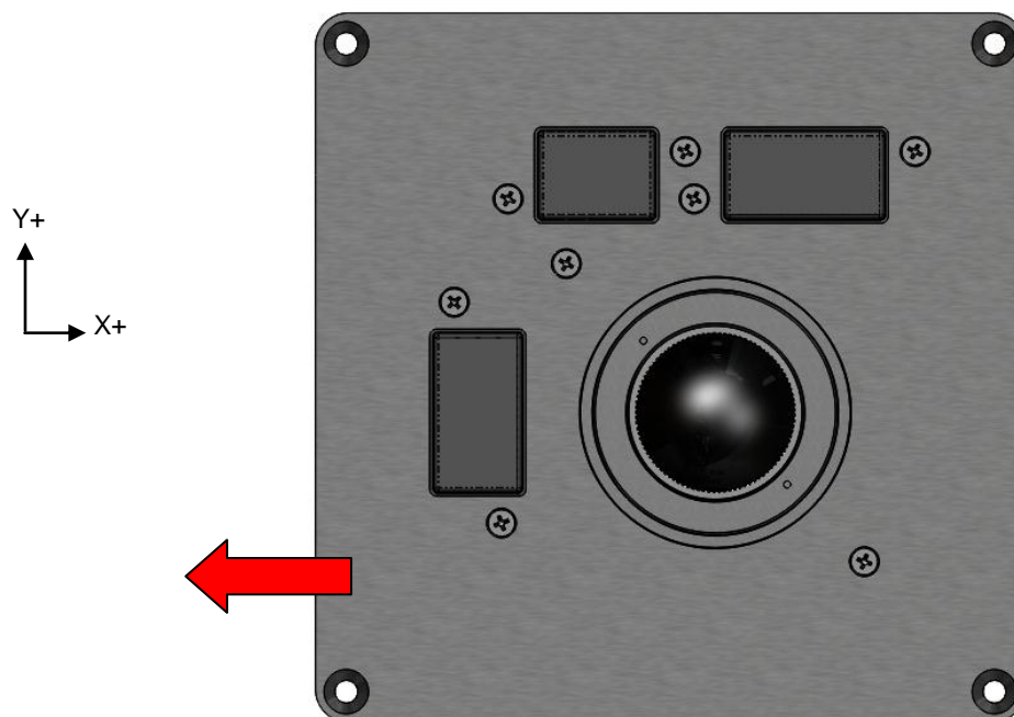
Figure 1 – Mounting Orientation
